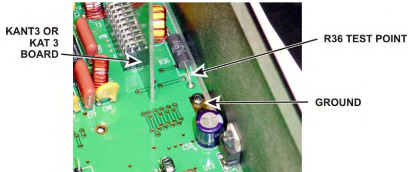
Figure 66. R36 Test Point.
