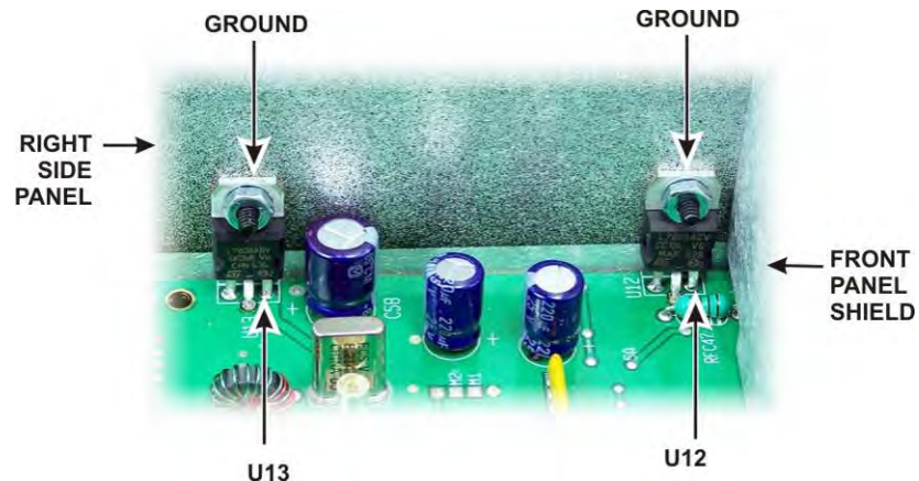
Figure 67. U12 and U13 Test Points.
